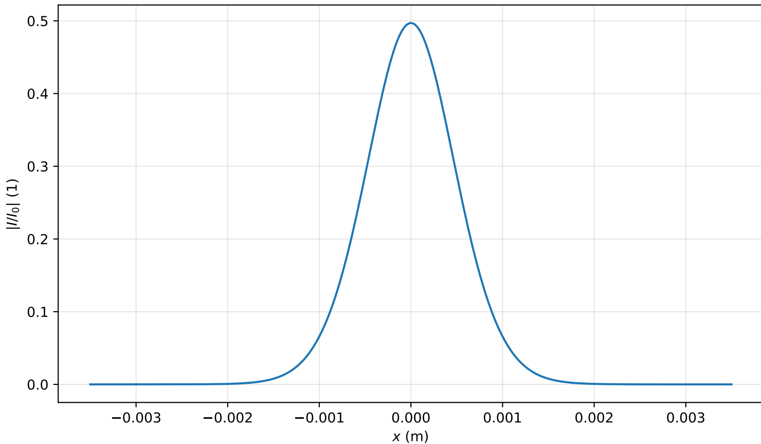
Intensity profile I(x, y = 0, z = 2.627m)/I_0 , P_{in}=0.3P_{cr} , artificial time
